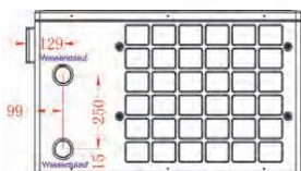
L x B x H = 968 x 360 x 584 (mm)
