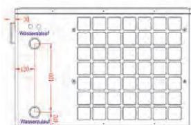
L x B x H = 1108 x 416 x 711 (mm)
