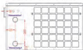
L x B x H = 1014 x 373 x 624 (mm)
